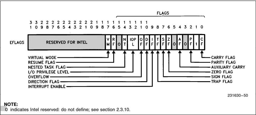
Figure 2-3. Flags Register
