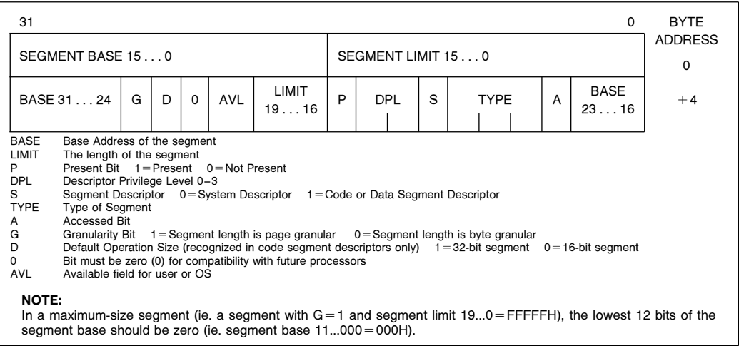
Figure 4-5. Segment Descriptors
